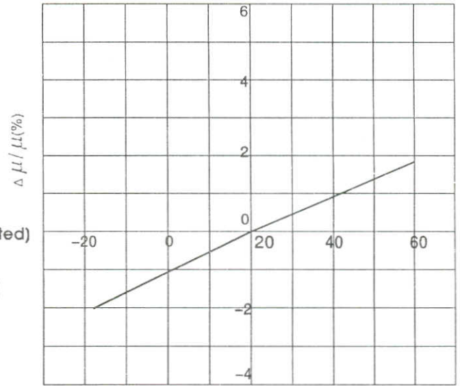
\Delta \mu / \mu Vs. temperature curve (M-series materials)
