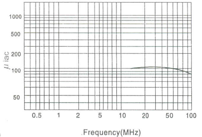
\mu_{iac} Vs. frequency response characteristics
